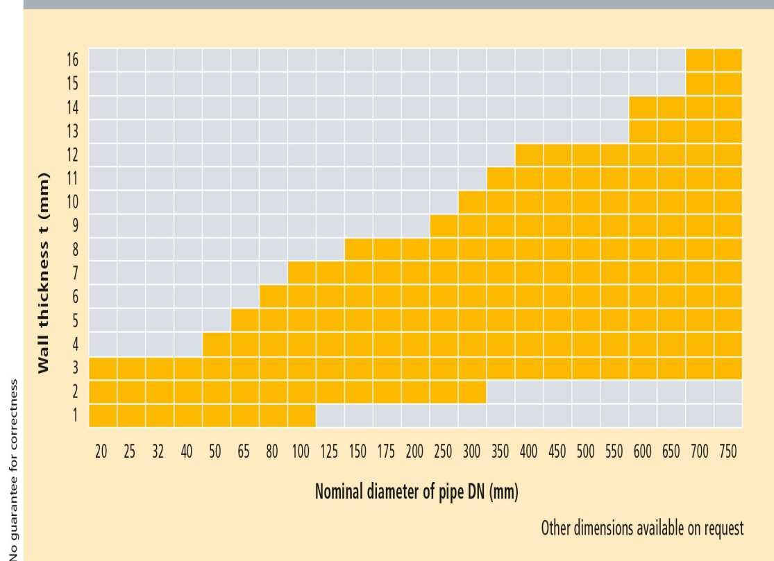
Fig. 1.1.2_1: Possible size range of pipes from coil
